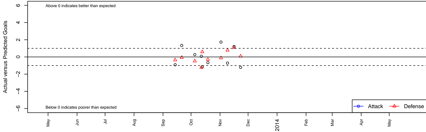
Central CA Soccer Alliance Black G00 Dots are actual minus expected GF (blue circles) and GA (red triangles). Blue line is smoothed change in attack strength. Red is smoothed change in defense strength.
